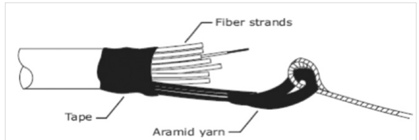
Drawing courtesy of BICSI® Information Technology Installation Methods Manual
